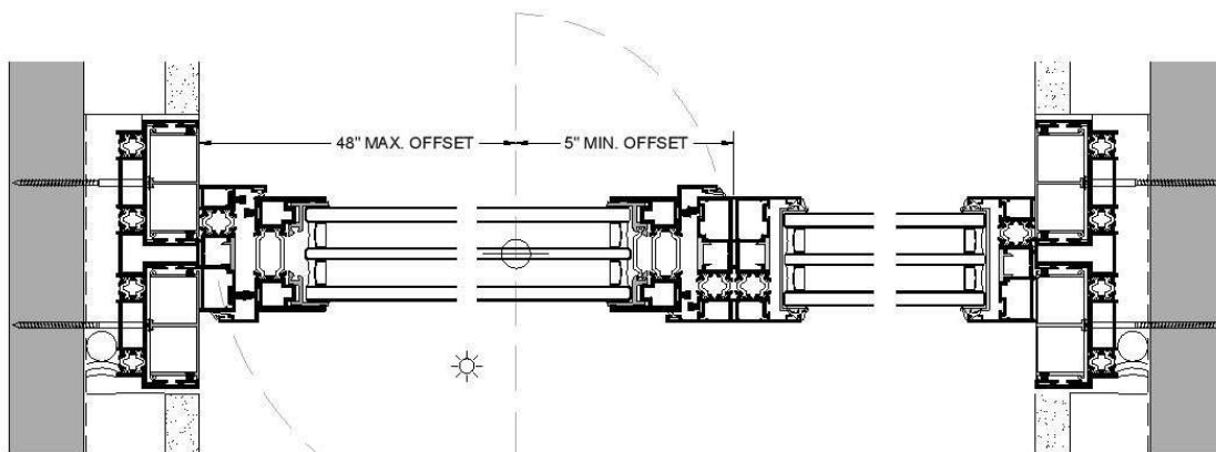
ELECTRONIC LOCKING STILE Magnetic Lock (12/24VDC)
