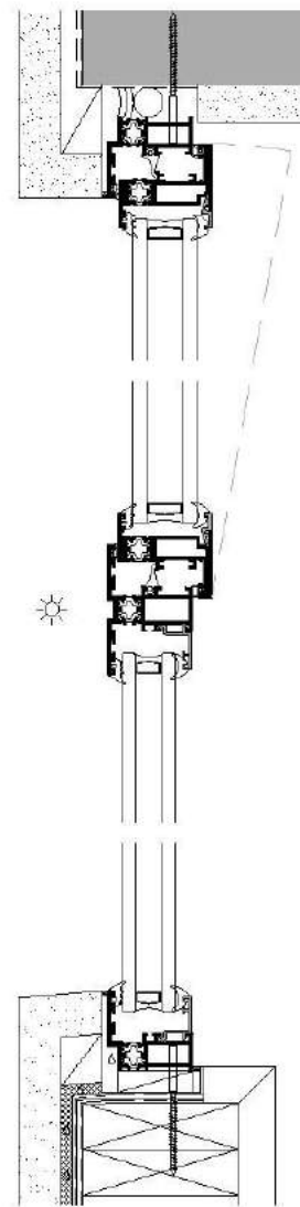
TILT/TURN OVER FIXED
