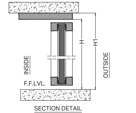
SECTION DETAIL
