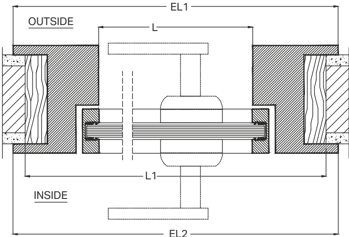
PLAN DETAIL
