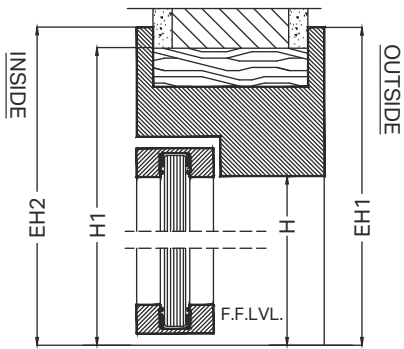
SECTION DETAIL
