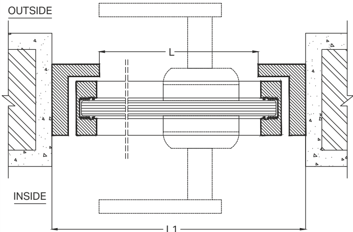
PLAN DETAIL
