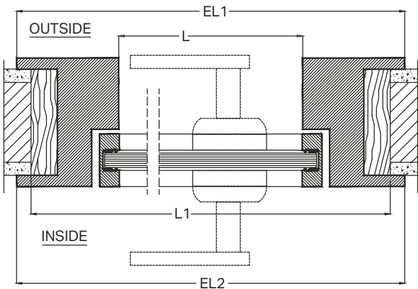
PLAN DETAIL
