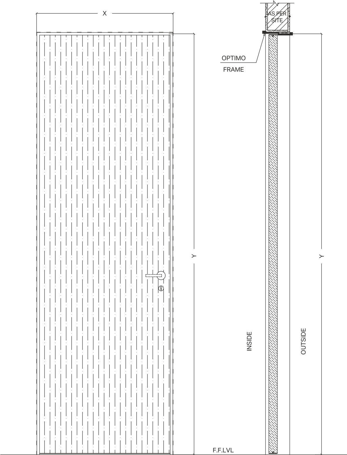
INSIDE ELEVATION
