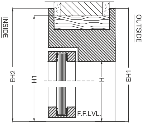
SECTION DETAIL
