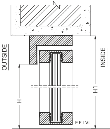
SECTION DETAIL
