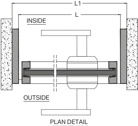
PLAN DETAIL
